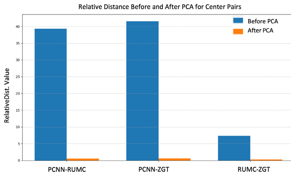
FIGURE 3 Relative distance between site centroids before and after applying FIPCA. Blue bars represent distances computed on standardized raw features, while orange bars show distances after FIPCA transformation. FIPCA, federated incremental principal component analysis.
