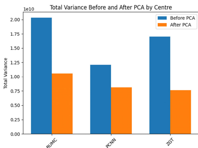
FIGURE 4 Total variance before and after FIPCA for each center. FIPCA, federated incremental principal component analysis.
