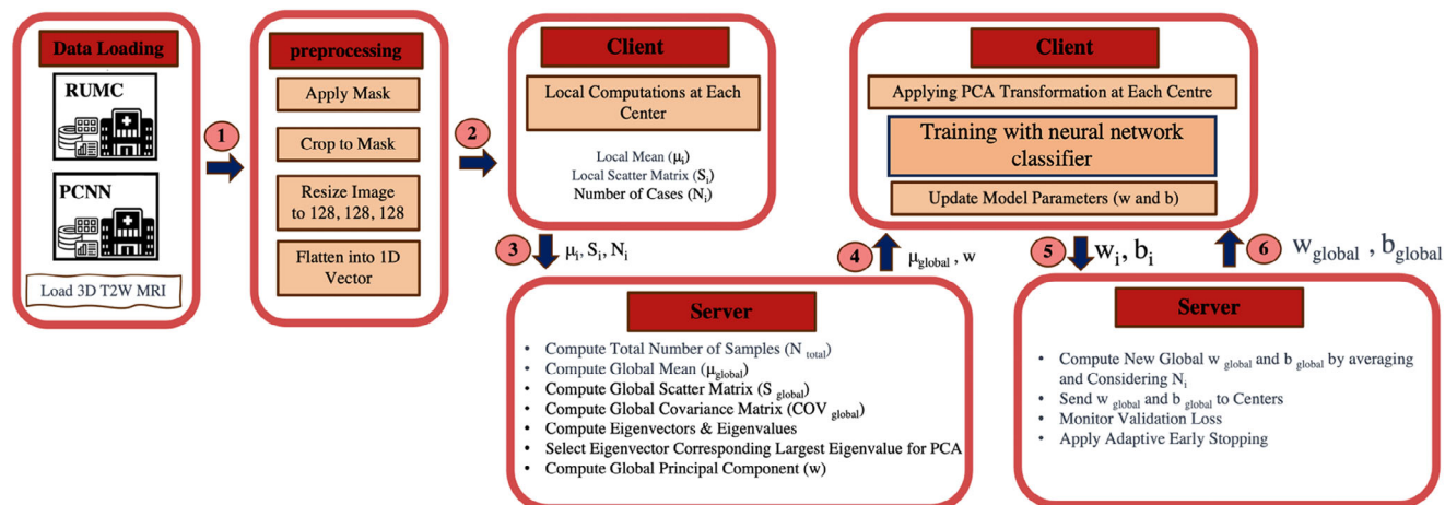
FIGURE 1 Our proposed adaptive process in a FL setup, illustrating federated data preprocessing, client-side adaptive training, and server-side coordination with an early stopping mechanism. Steps 5 and 6 repeat as rounds between clients and the server until the convergence criteria are met. FL, federated learning.
