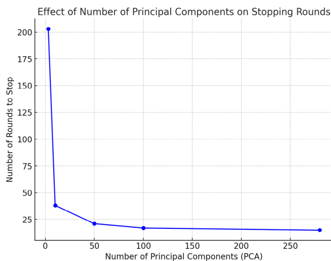
FIGURE 6 Effect of FIPCA component count on training rounds. FIPCA, federated incremental principal component analysis.
